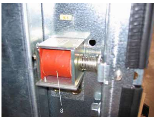
fig. 23 – Internal view
