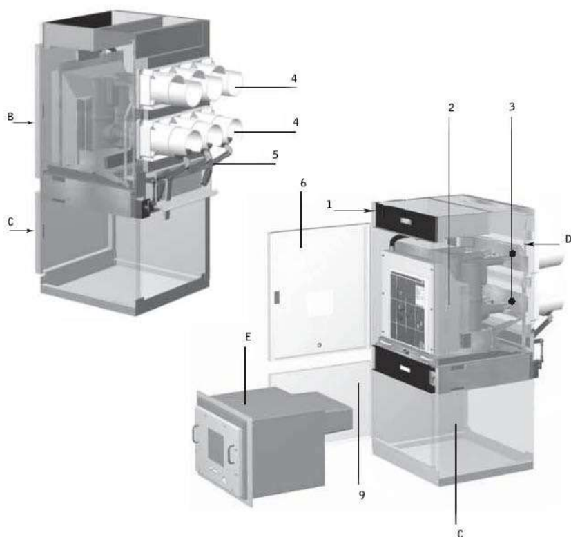
fig. 7 – Typical section
